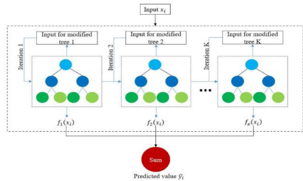
FIGURE 3. Fundamental structure of XGBoost.
