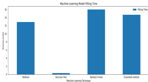
FIGURE 8. ML model training time.
