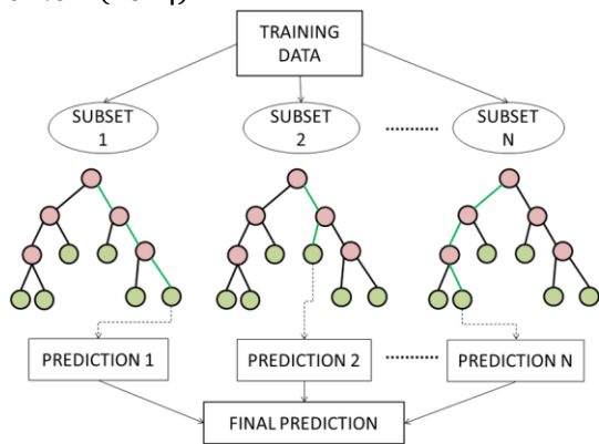
FIGURE 2. Fundamental concept of a RF model.
