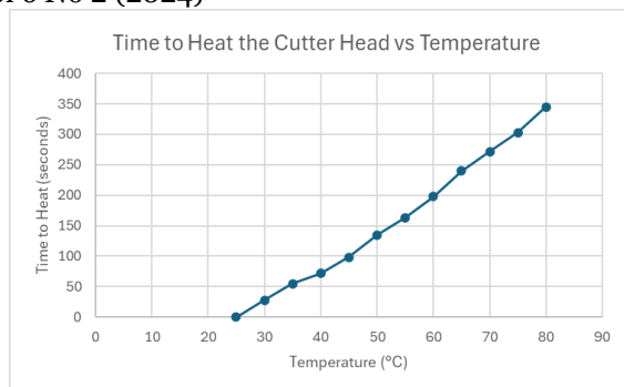
FIGURE 5. Time to heat the cutter head against temperature.
