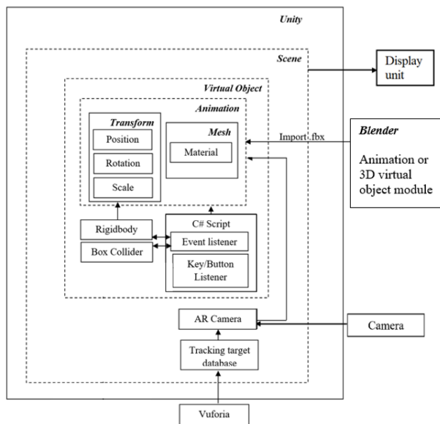
Figure 3. System Configuration
