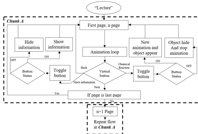
Figure 7. The "Lecture" mode Flow Chart
