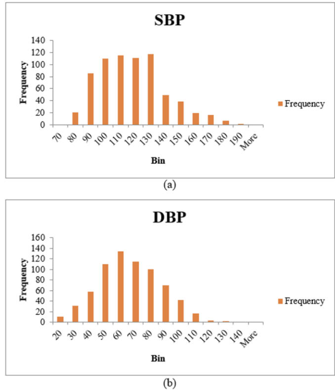
Figure 1. Data distribution in MIMIC-II Dataset for (a) SBP and (b) DBP
