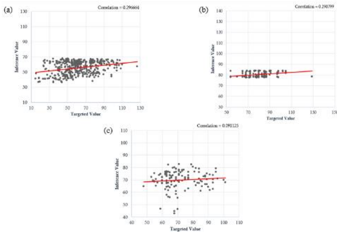
Figure 6. Correlation graph of DBP for (a) MIMIC-II, (b) UKM, and (c) PPG-BP Dataset
