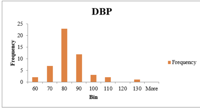
Figure 2. Data distribution in UKM Dataset for (a) SBP and (b) DBP
