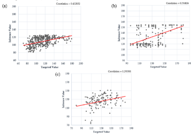
Figure 5. Correlation graph of SBP for (a) MIMIC-II, (b) UKM, and (c) PPG-BP Dataset
