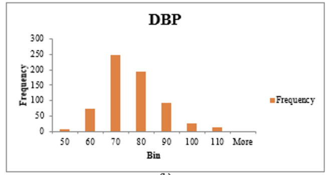
Figure 3. Data distribution in PPG-BP Dataset for (a) SBP and (b) DBP
