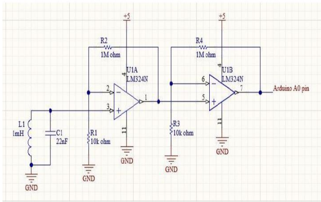
FIGURE 5(A). The Im324n amplification schematic.
