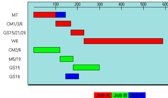
Fig. 4. Gantt chart of best schedule for (E + T)_{\min} (Case 1).
